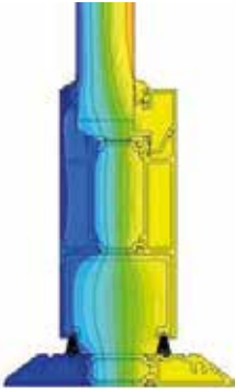
Isotherm image of single door open but out rebated door
